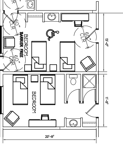
TYPICAL BEDROOMS SCALE: 1/4" = 1'-0"
